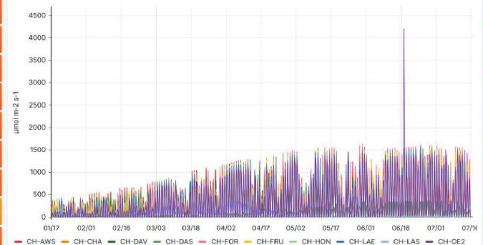
Photosynthetically Active Radiation (μmol m -2 s -1 )
